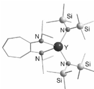
Fig. 5 Crystal structure of 13 .
